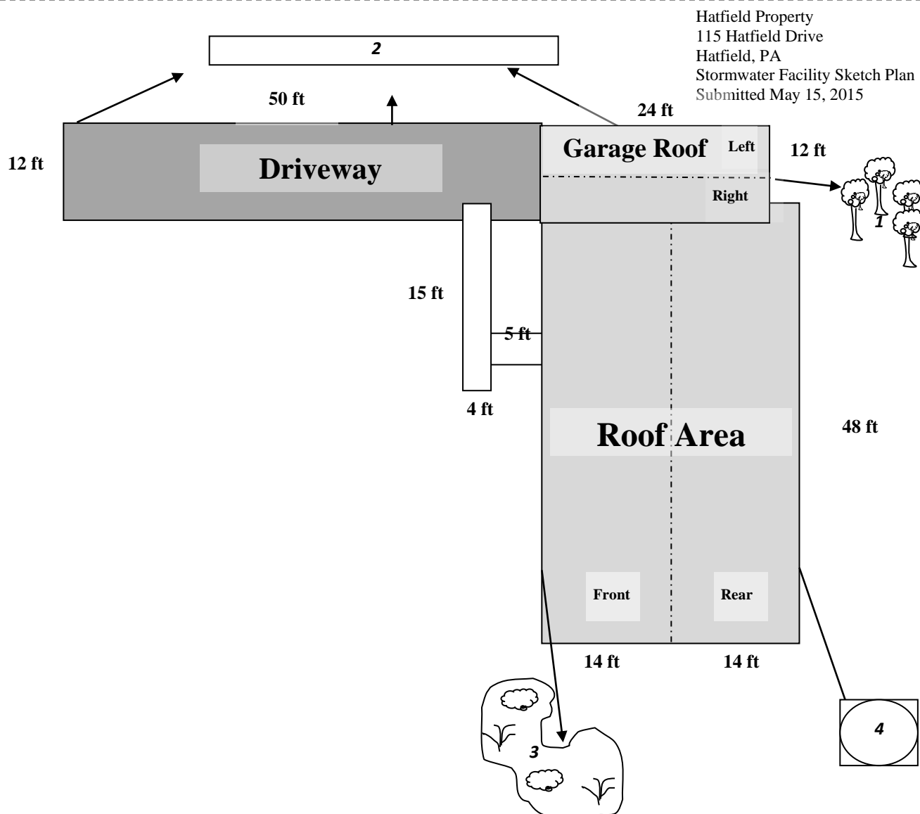
Figure 1: Sample Site Sketch Plan (Note: Figure 1 is an example of how various BMPs can be utilized in conjunction to control the total required volume on one site.)
